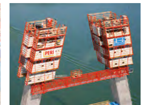
Through the catwalk between the pylons, only one elevator was required which greatly reducing the amount of walking for site personnel. The catwalk was always positioned horizontally regardless of the angle of the climbing formwork units.
