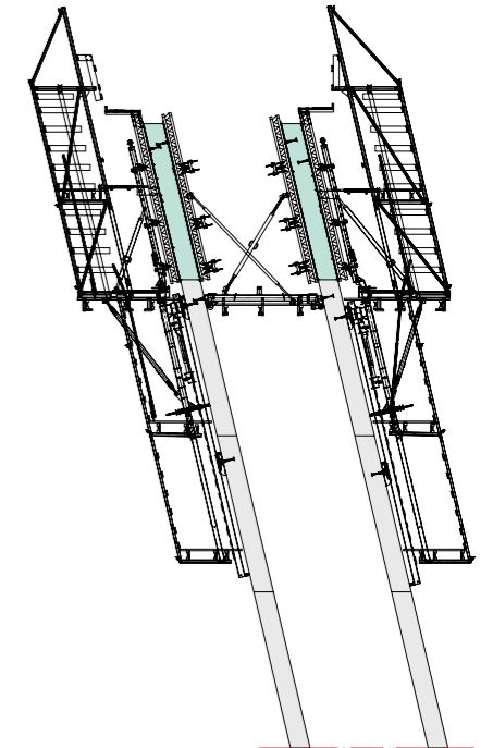
The adjustable ACS V self-climbing system was the ideal solution for the inclined pylon supporting members.
